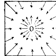
Fig. 8 Sequential reaction
